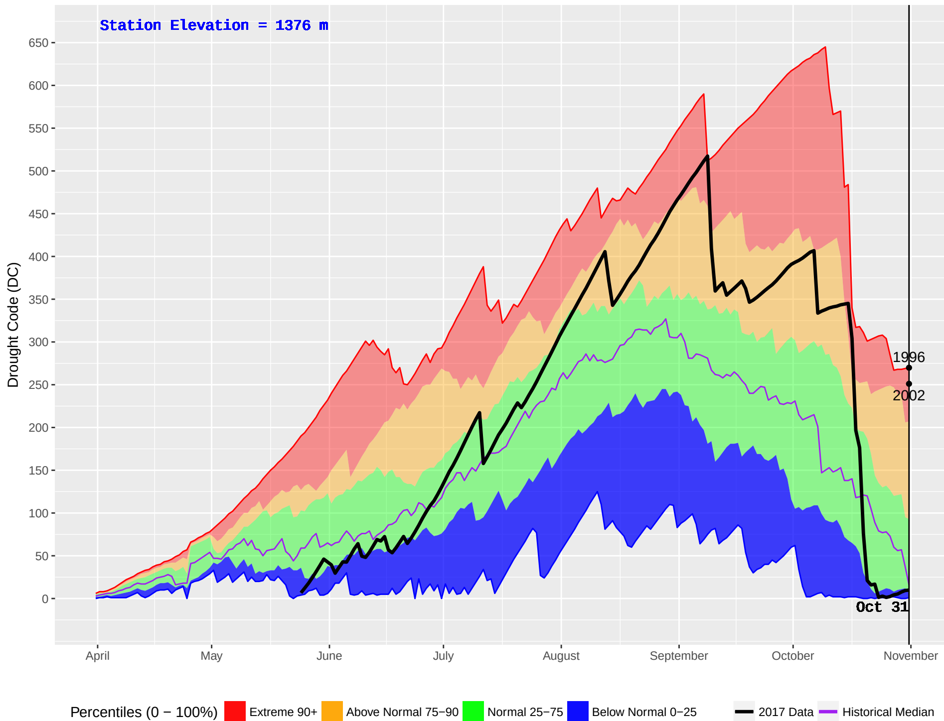
DUNCAN (385) : Historical (1981–2016) and Current (2017) Noon Drought Code (DC)
