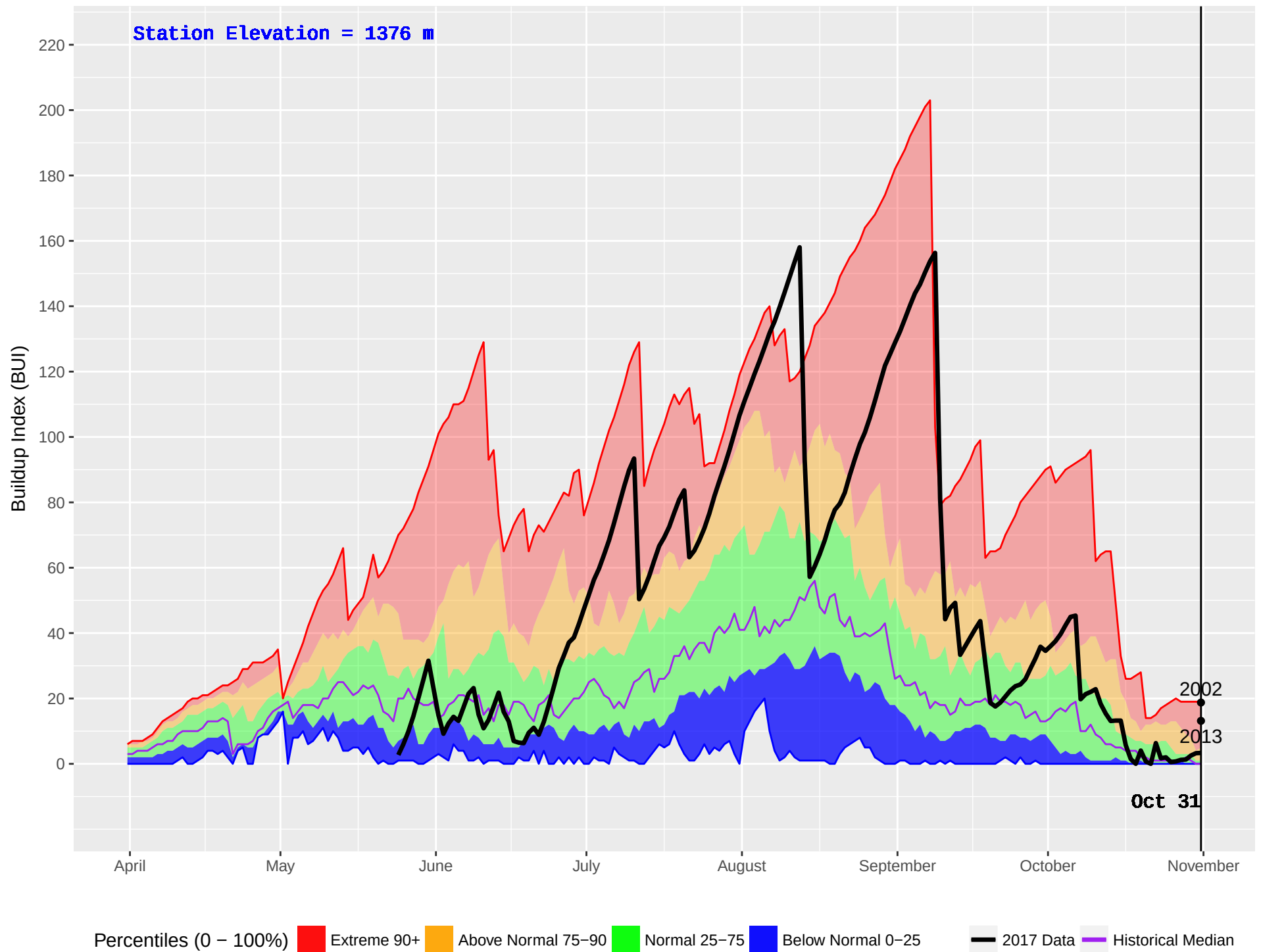
DUNCAN (385) : Historical (1981–2016) and Current (2017) Noon Buildup Index (BUI)
